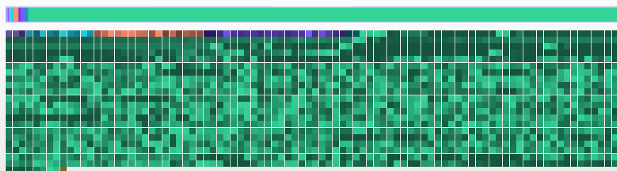
PACKET BITS
